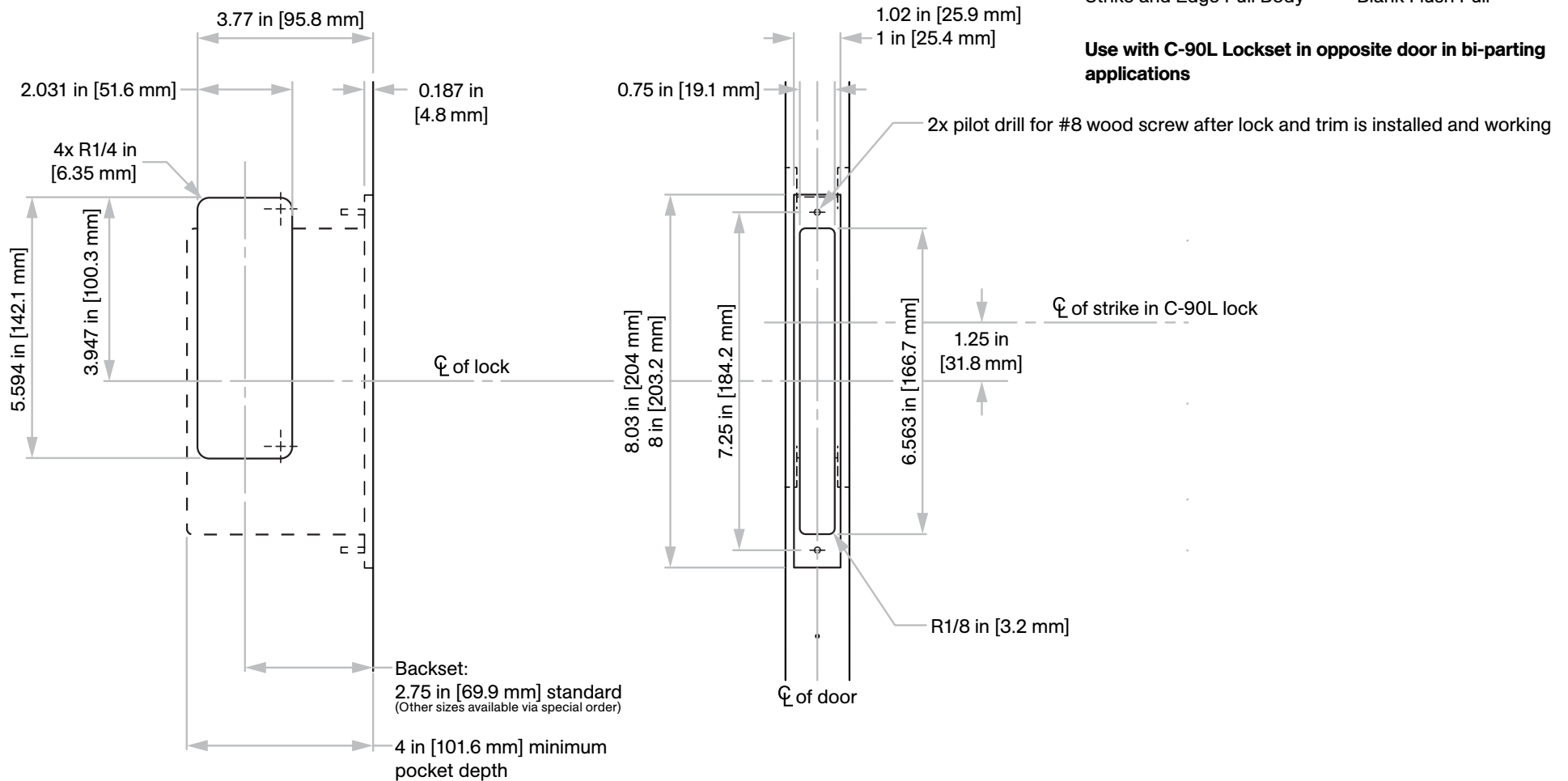
C-90S Strike and Edge Pull Body
