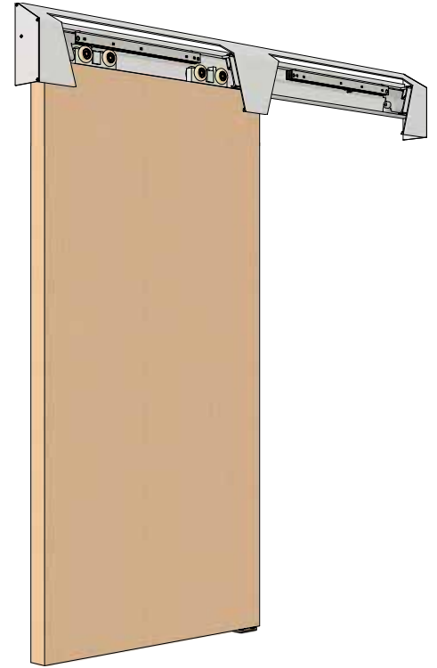
Complete CCSSF-810 kit illustrated. Cut-outs in track to expose components.
